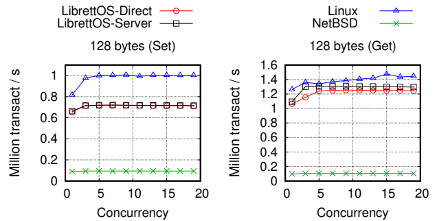
Figure 12. Redis key-value store.
