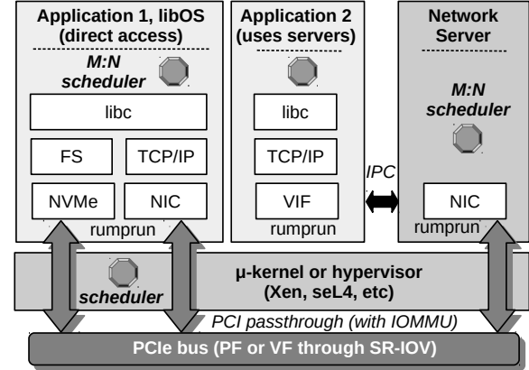
Figure 3. LibrettOS’s architecture.
