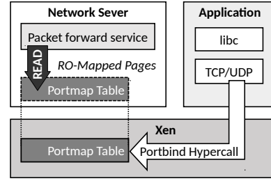
Figure 5. Portmap table.
